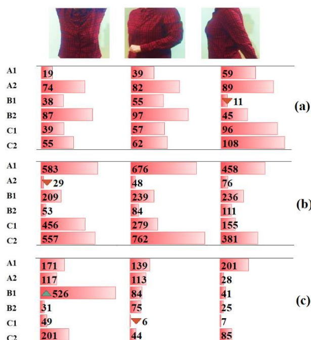
Figure 1: Slope Values of the Voltage-Time Diagram (10000×) During Various Movements: A) Metal Thread at the Bottom Of The Cup, B) Metal Thread at the Bottom of the Back Band, (C) Metal Thread At the Bottom of the Middle Triangle
